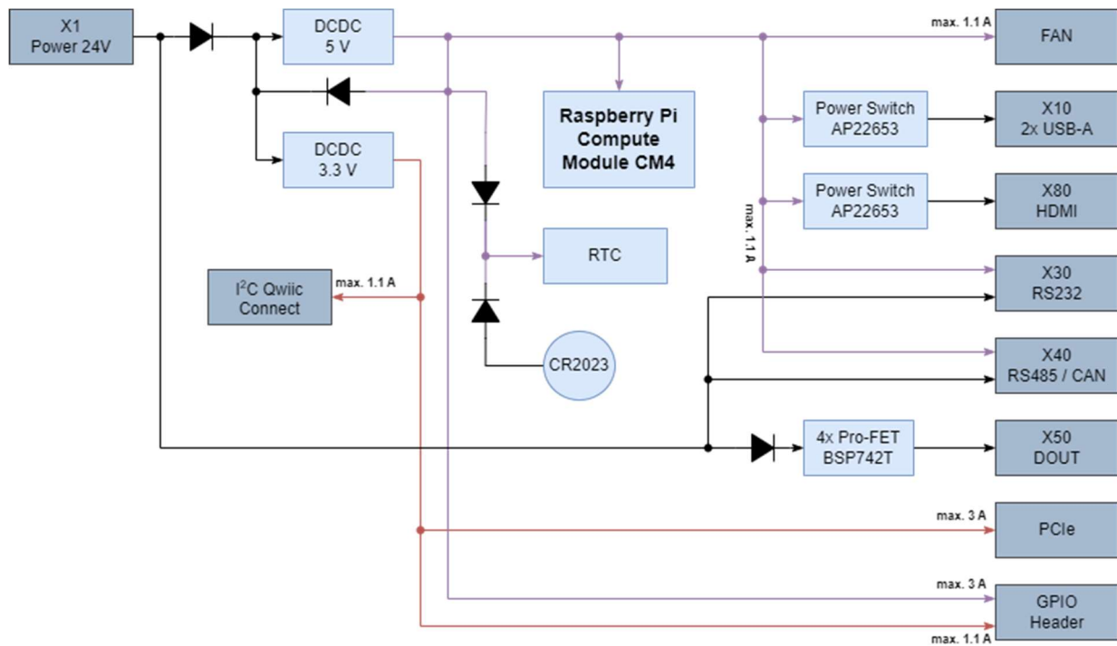
Figure 6: Power Tree
