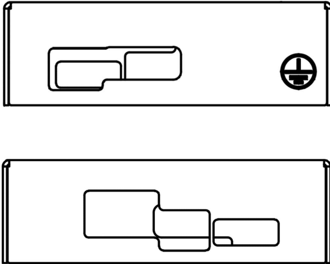
Figure 5: Side views
