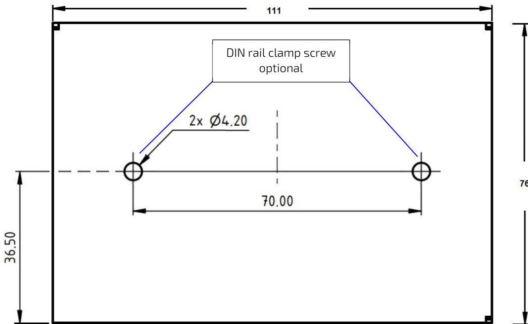
Figure 2: Bottom view
