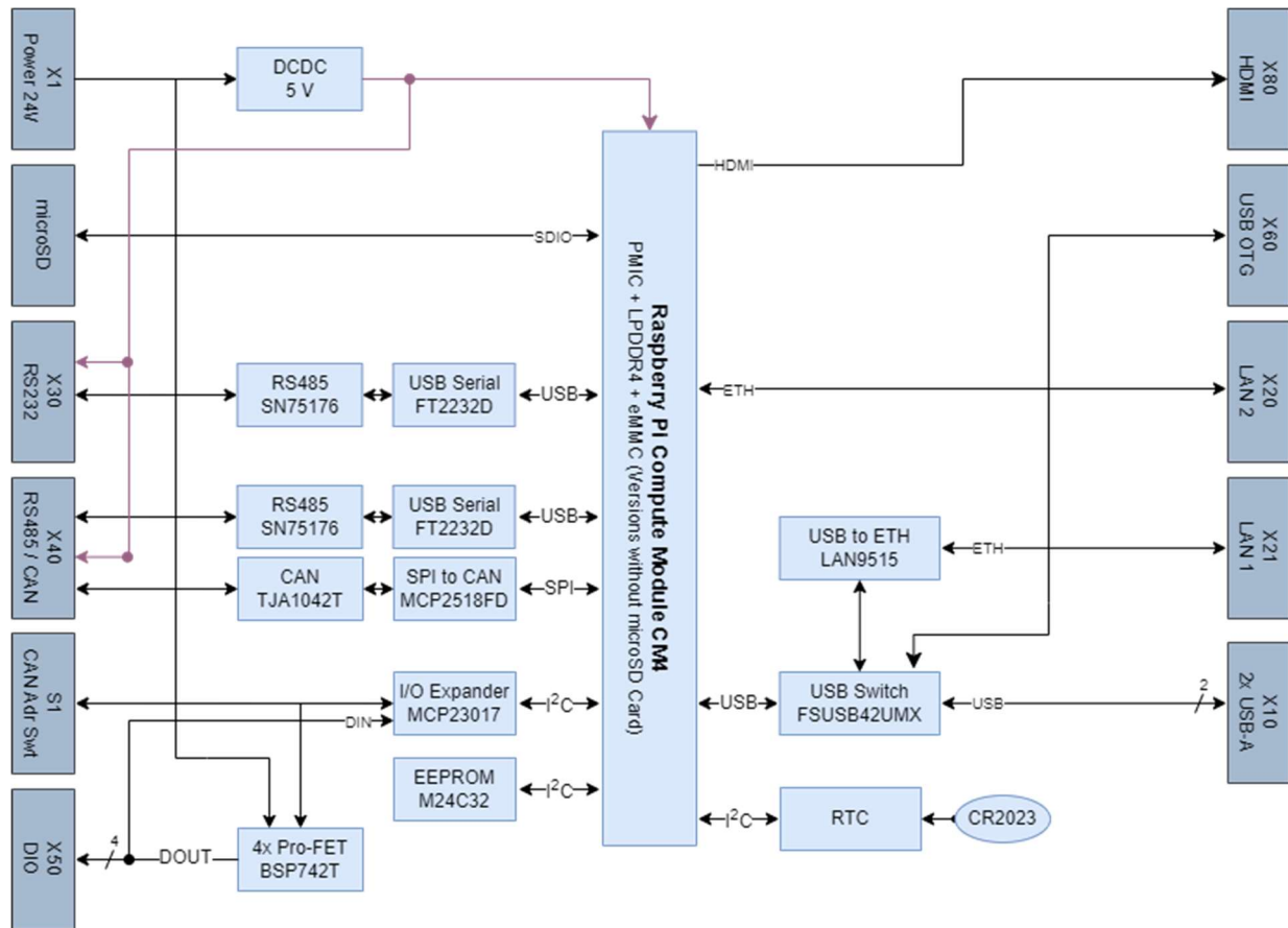
Figure 7: Block Diagram
